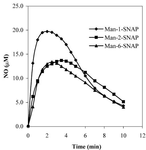
Figure 3. NO generation by a 0.2 mM solution of mannose SNAPs in a phosphate buffer (0.1 M, pH 7.4) and 50 μM Cu 2+ .
