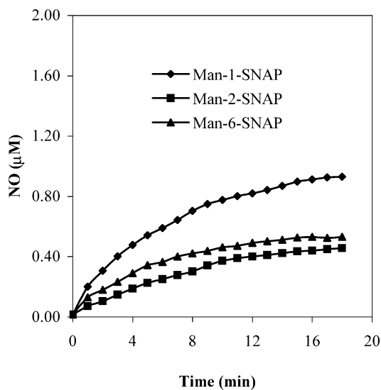
Figure 2. NO generation by a 0.2 mM solution of mannose SNAPs in a phosphate buffer (0.1 M, pH 7.4) and 1.0 mM EDTA.
