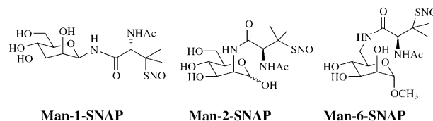
Figure 1. Structures of Man-SNAPs.
