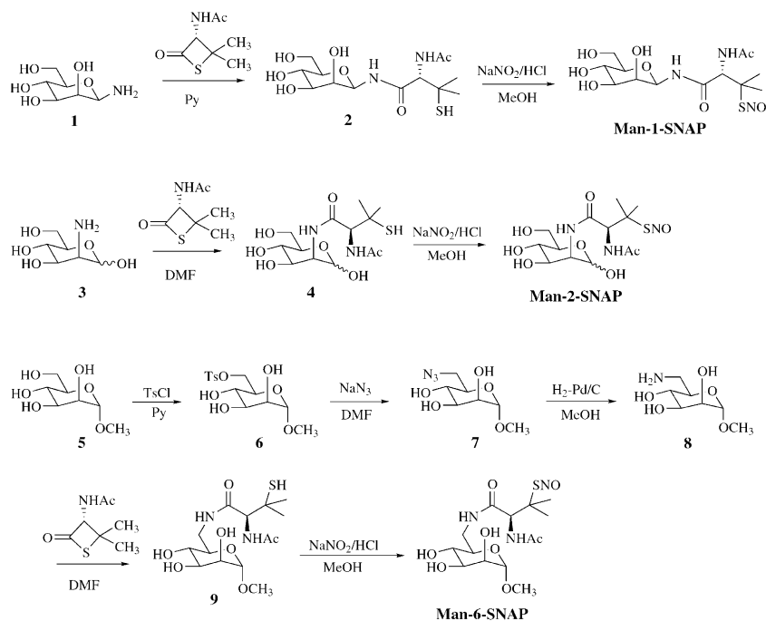
Scheme 1. Synthetic methodology toward Man-1-SNAP, Man-2-SNAP, and Man-6-SNAP.
